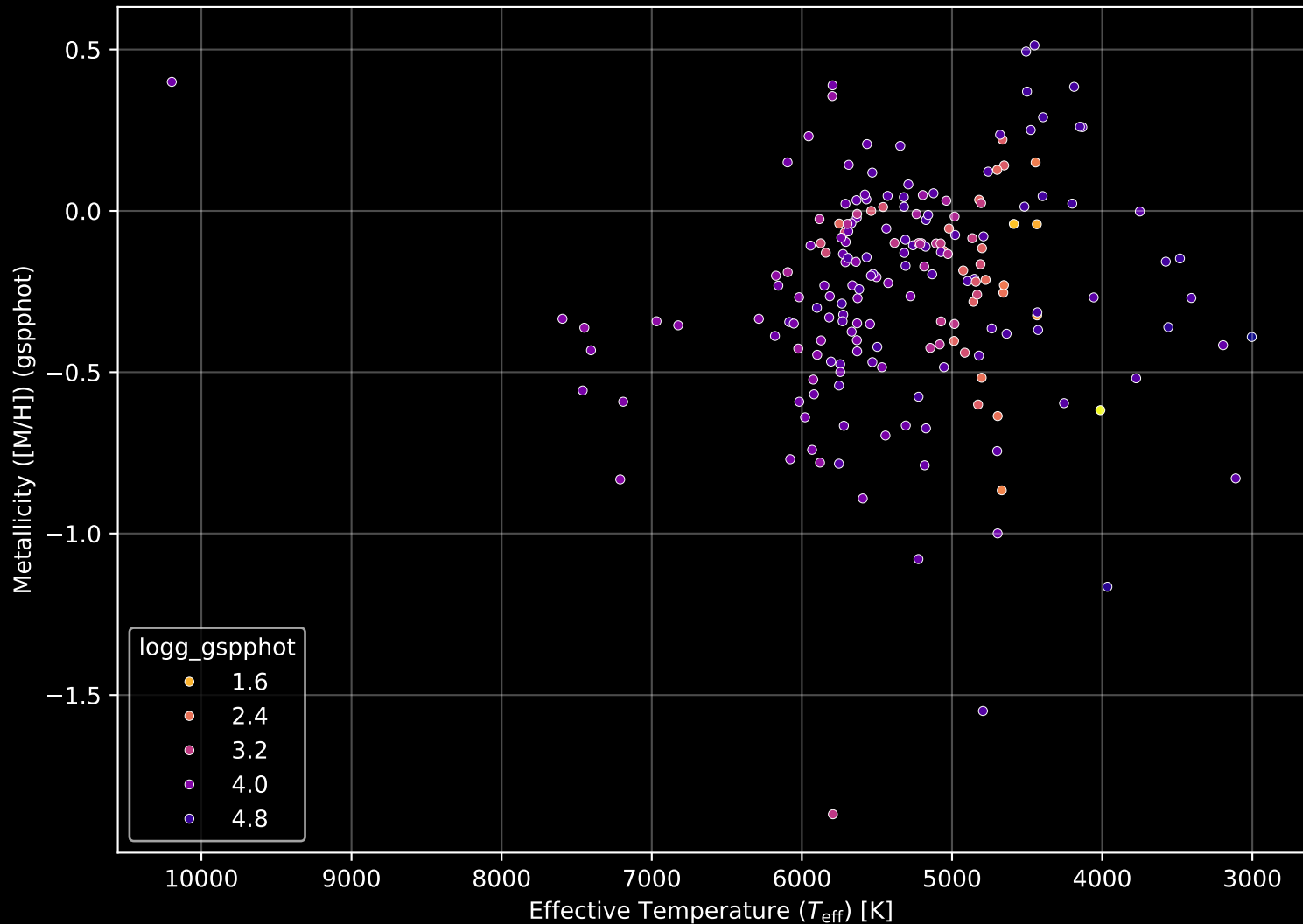
APOGEE DR17 Field: [172+34_MGA] Stellar Population Parameters (n= 193)
