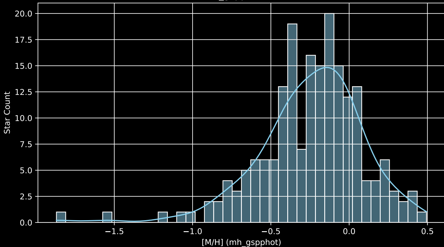
APOGEE DR17 Field: [172+34_MGA [M/H] (mh_gspphot) (n= 192)
