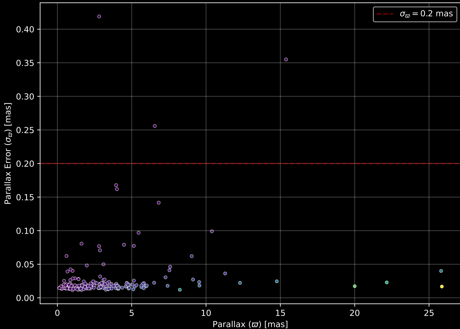
APOGEE DR17 Field: [172+34_MGA] Parallax Quality (n= 193)
