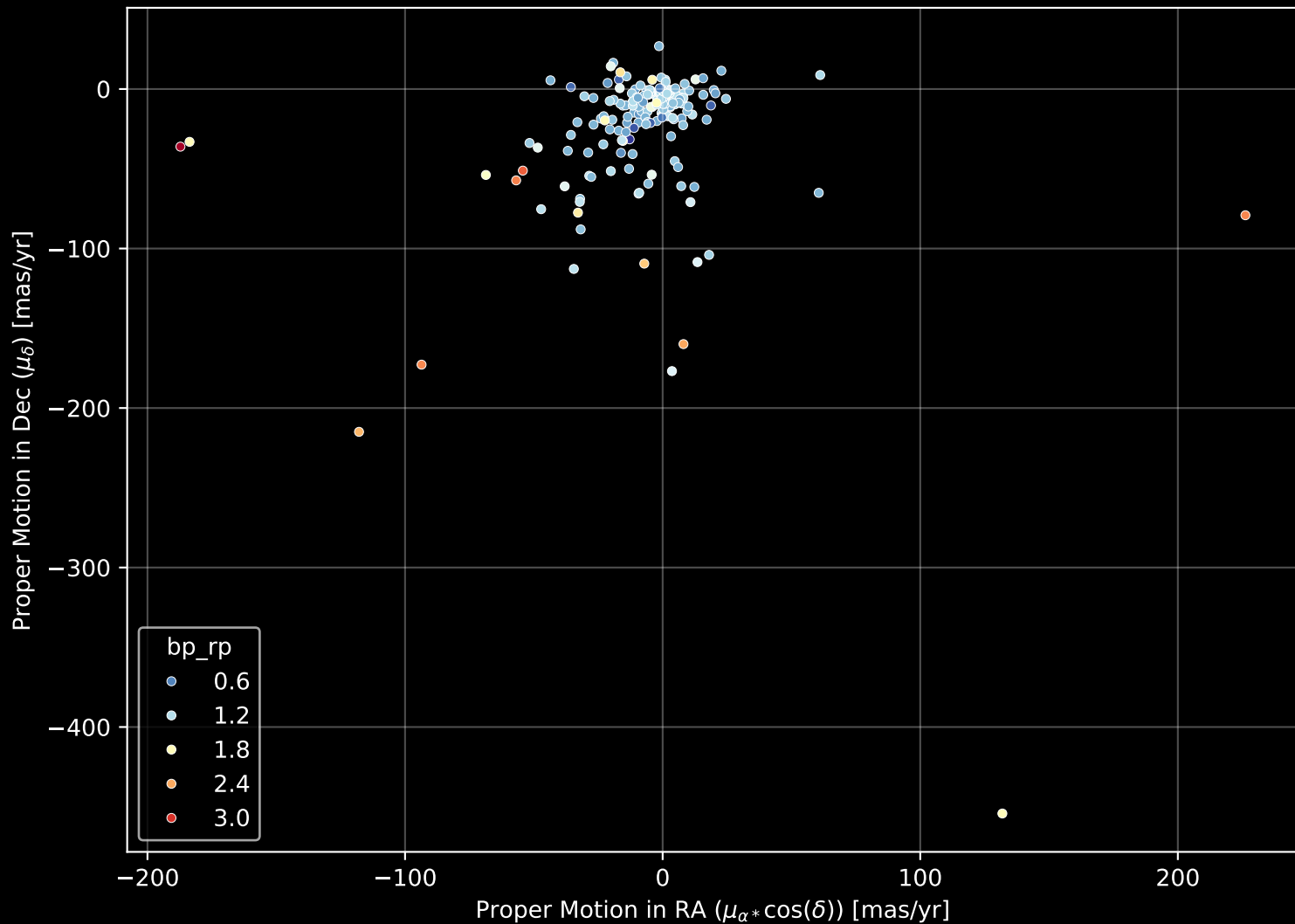
APOGEE DR17 Field: [172+34_MGA] Proper Motion Diagram (n= 193)
