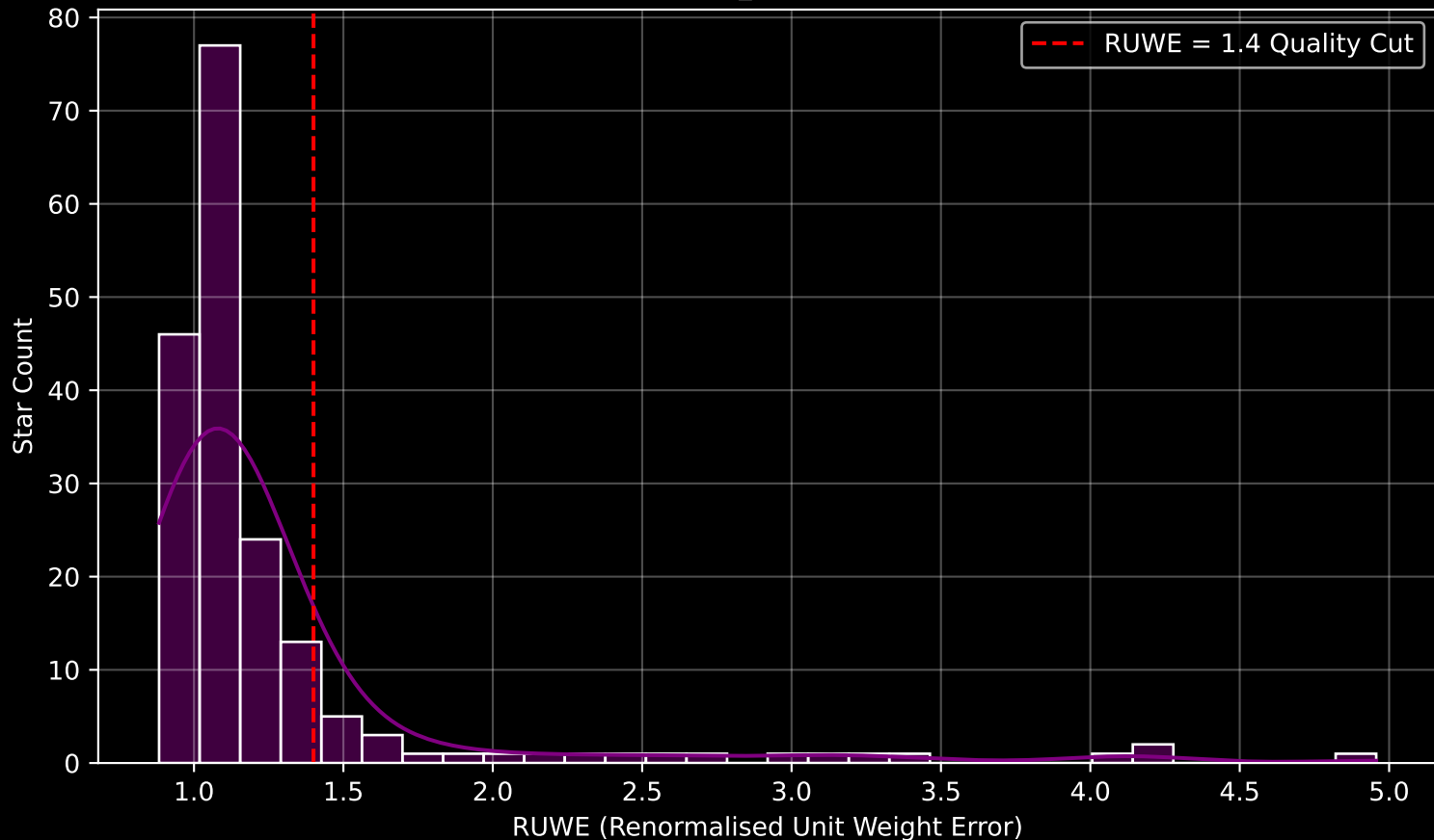
GAPOGEE DR17 Field [172+34_MGA] RUWE Distribution (n= 184)
