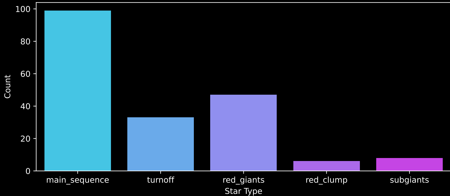
APOGEE DR17 Field: [172+34_MGA] Count plot of Star Type
